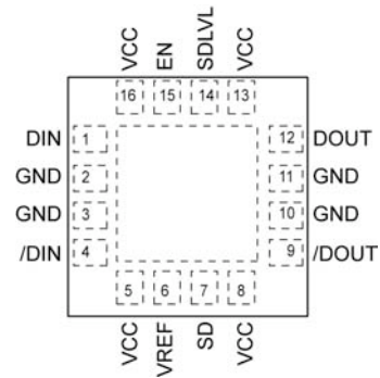
16-Pin MLF® (MLF-16)
